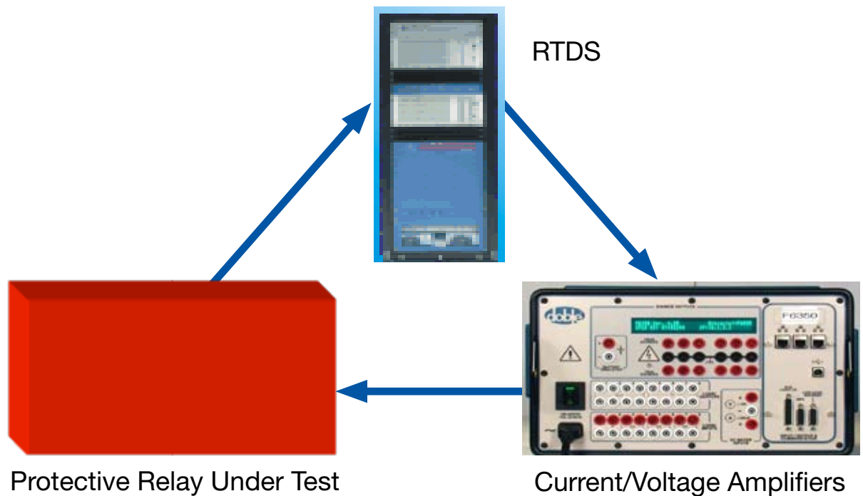
Figure 1: Closed Loop Real Time Testing
