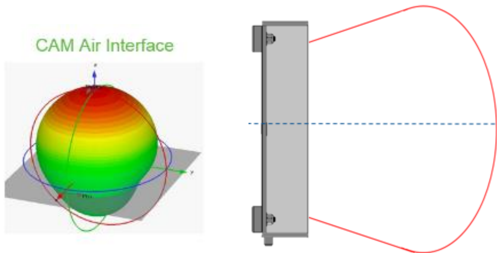
Figure 20: (Left) Air Interface Radiation Pattern. (Right) Pattern Relative to Air Interface
