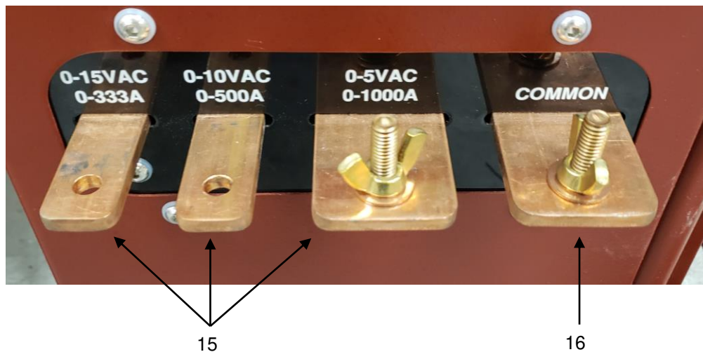
Figure 3: Output Taps
