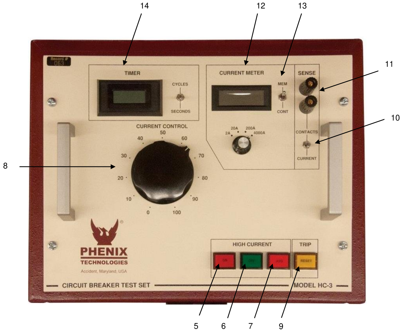
Figure 2. HC-3 Controls and Indicators
