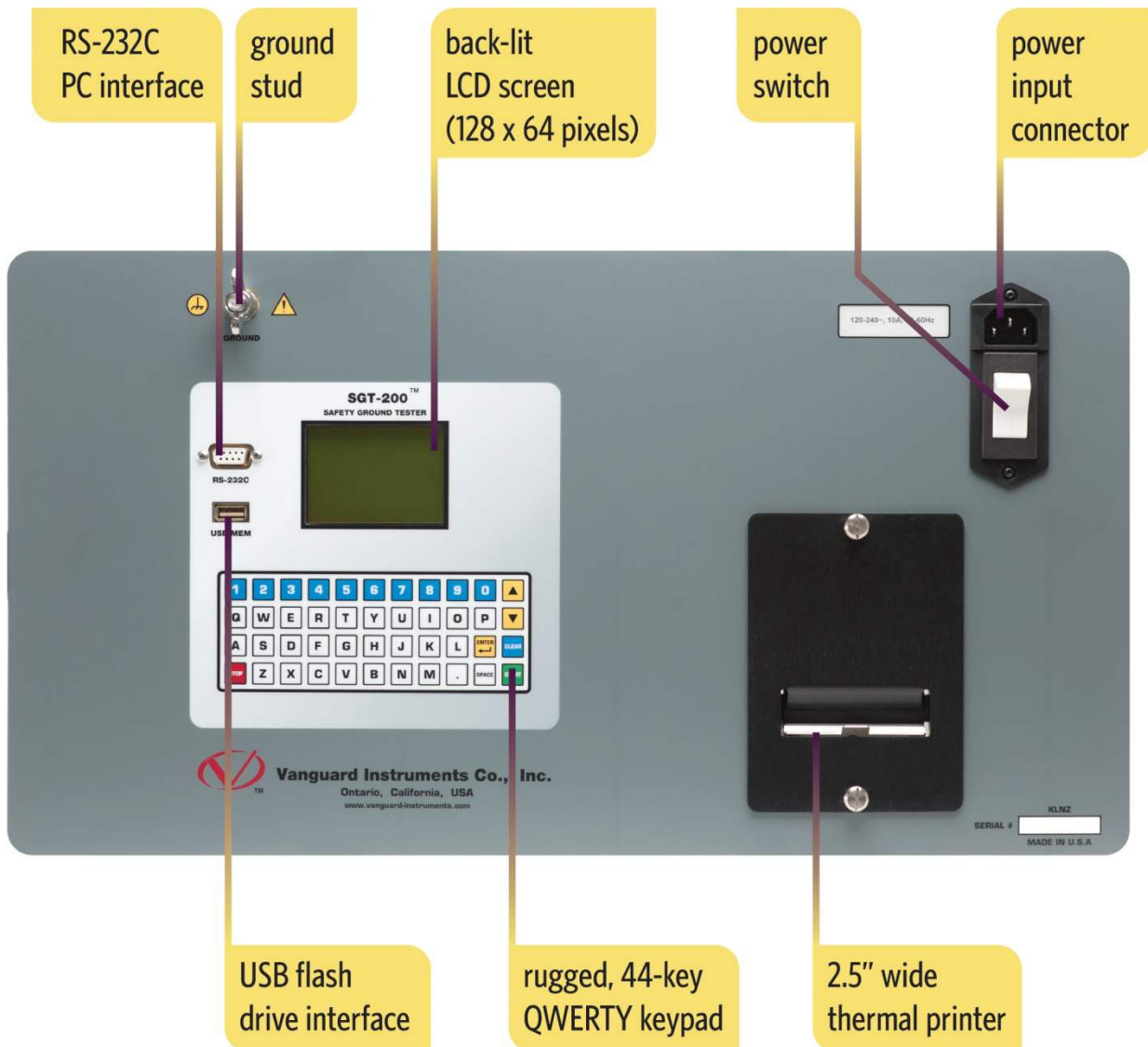
Figure 1. SGT-200 Controls and Indicators
