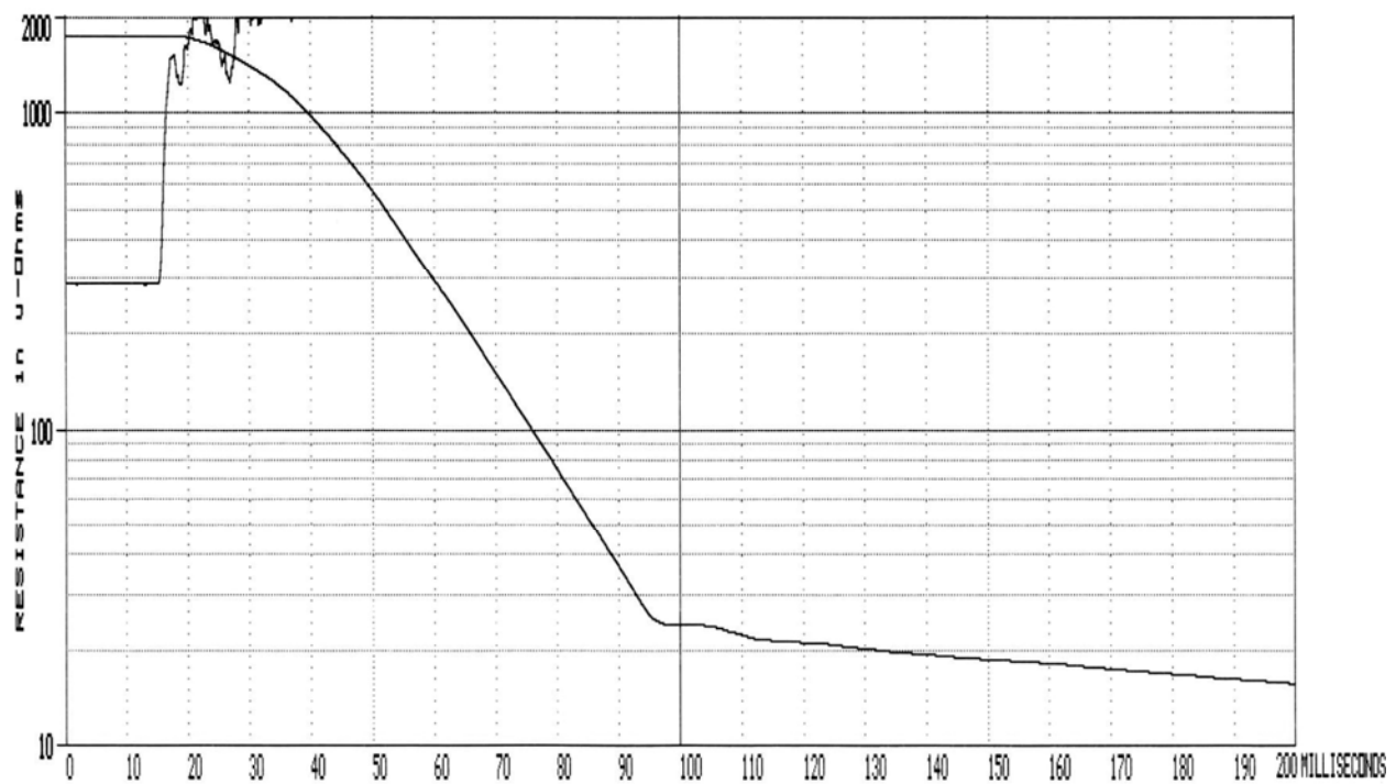
Figure 26. Dynamic Resistance Graph in Semi-Log Scale
