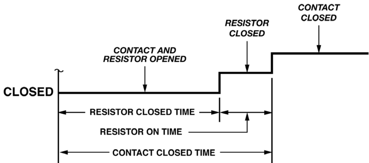
Figure 33. Graphical Interpretation of a CLOSE Timing Shot
