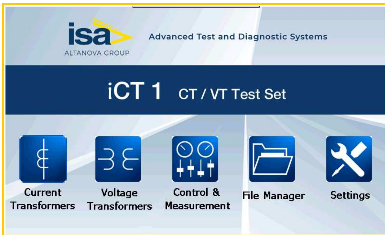
Figure 4 Home page
