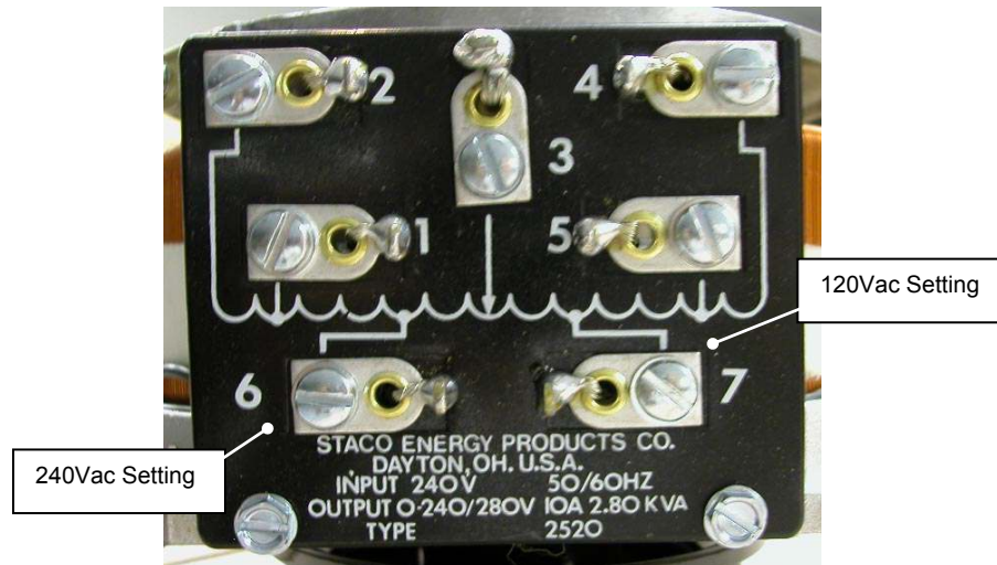
Figure 3 Variac Terminals
